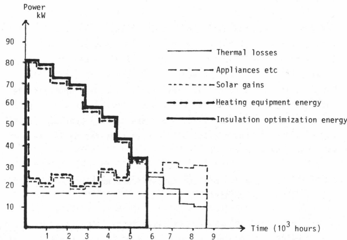
Figure 1: Duration curve for residential heating
