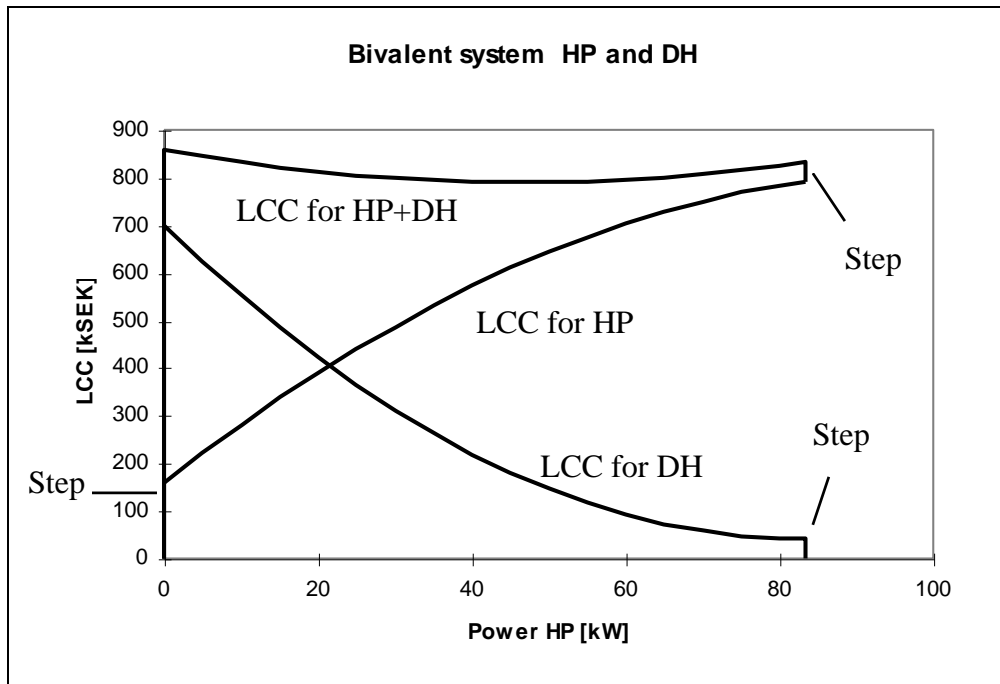
Diagram 7. LCC for a heat pump and district heating, with marginal cost pricing.
