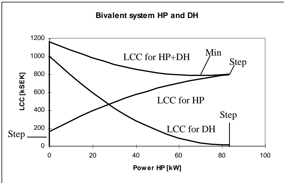
Diagram 6. LCC for a heat pump and district heating, with the district heating tariff
