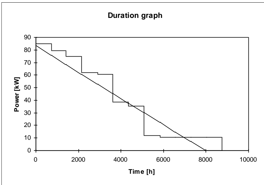
Diagram 5. Duration graph for the heating season, also showing the linear regression line
