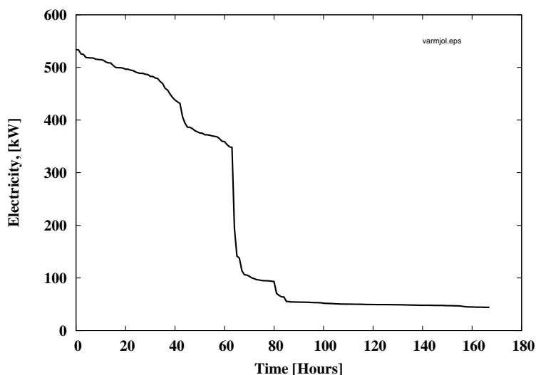
Figure 4: Electricity demand in the Mjölby factory from 13 to 20 September 1994
