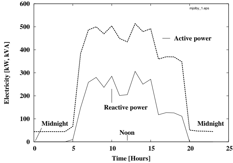
Figure 3: Electricity demand at Klintland AB in Mjölby, during 13 September 1994.
