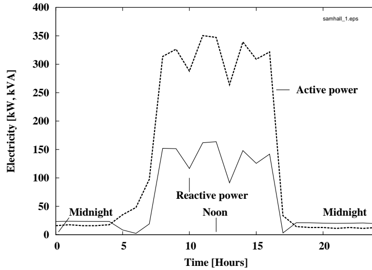
Figure 2: Electricity demand at Klintland AB, Linköping, during 19 September 1994.
