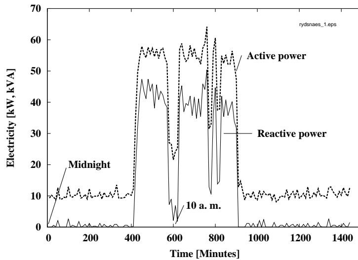
Figure 1: Electricity supplied to Rydsnäs Carpentry AB during 21 March 1994
